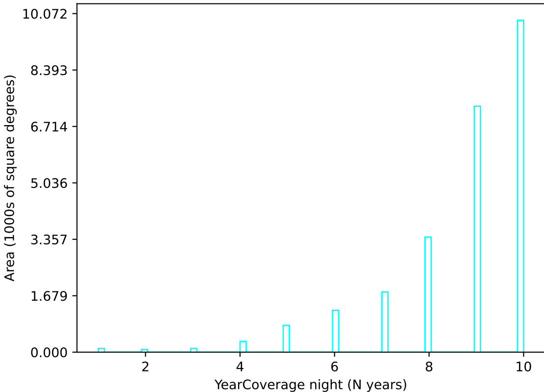
scp_reweight_v3.3_10yrs u band: YearCoverage night
