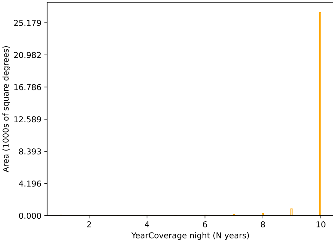
scp_reweight_v3.3_10yrs r band: YearCoverage night
