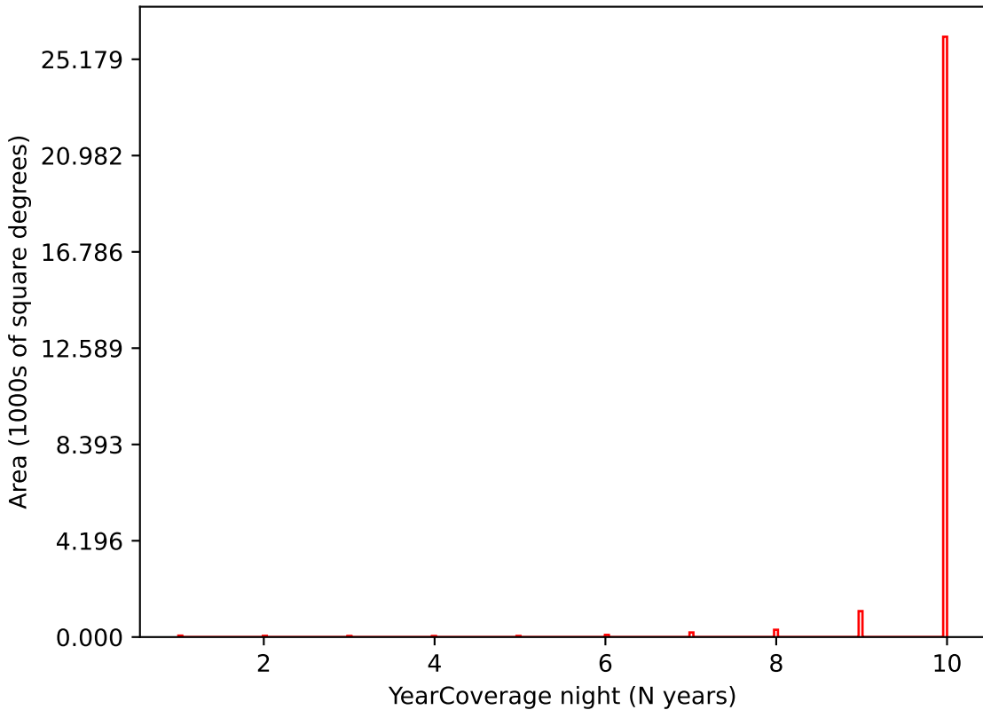
scp_reweight_v3.3_10yrs i band: YearCoverage night
