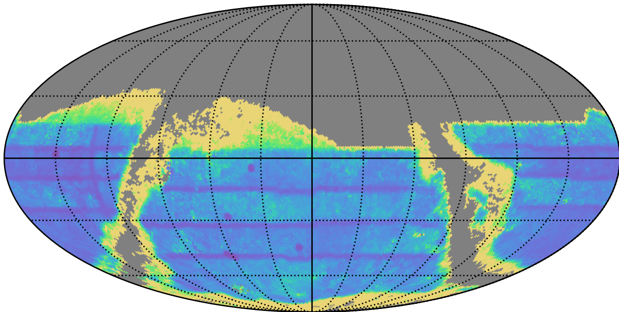
scp_reweight_v3.3_10yrs : TDC_precision
