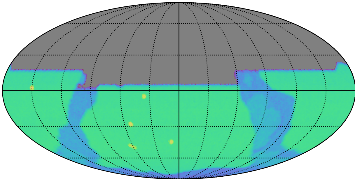
scp_reweight_v3.3_10yrs y: SurfaceBrightLimit
