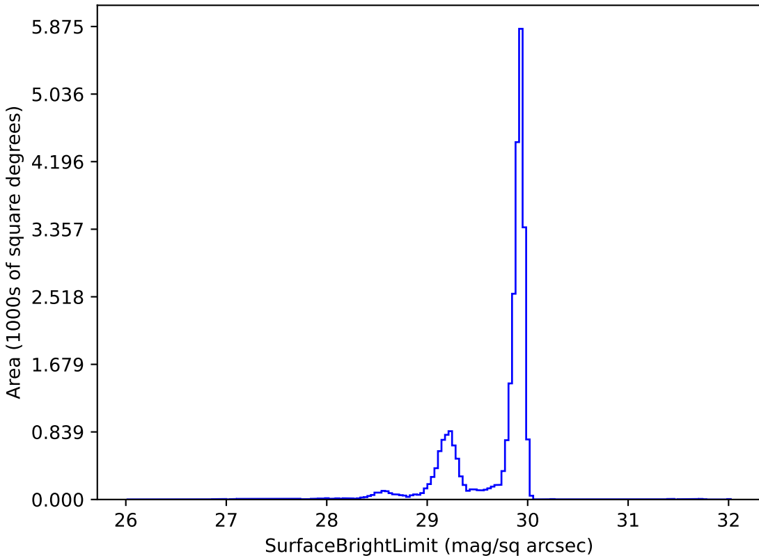
scp_reweight_v3.3_10yrs i: SurfaceBrightLimit
