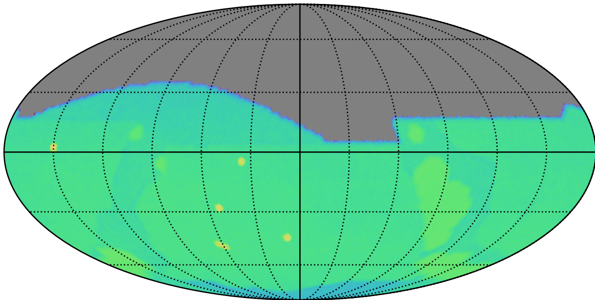
scp_reweight_v3.3_10yrs g: SurfaceBrightLimit
