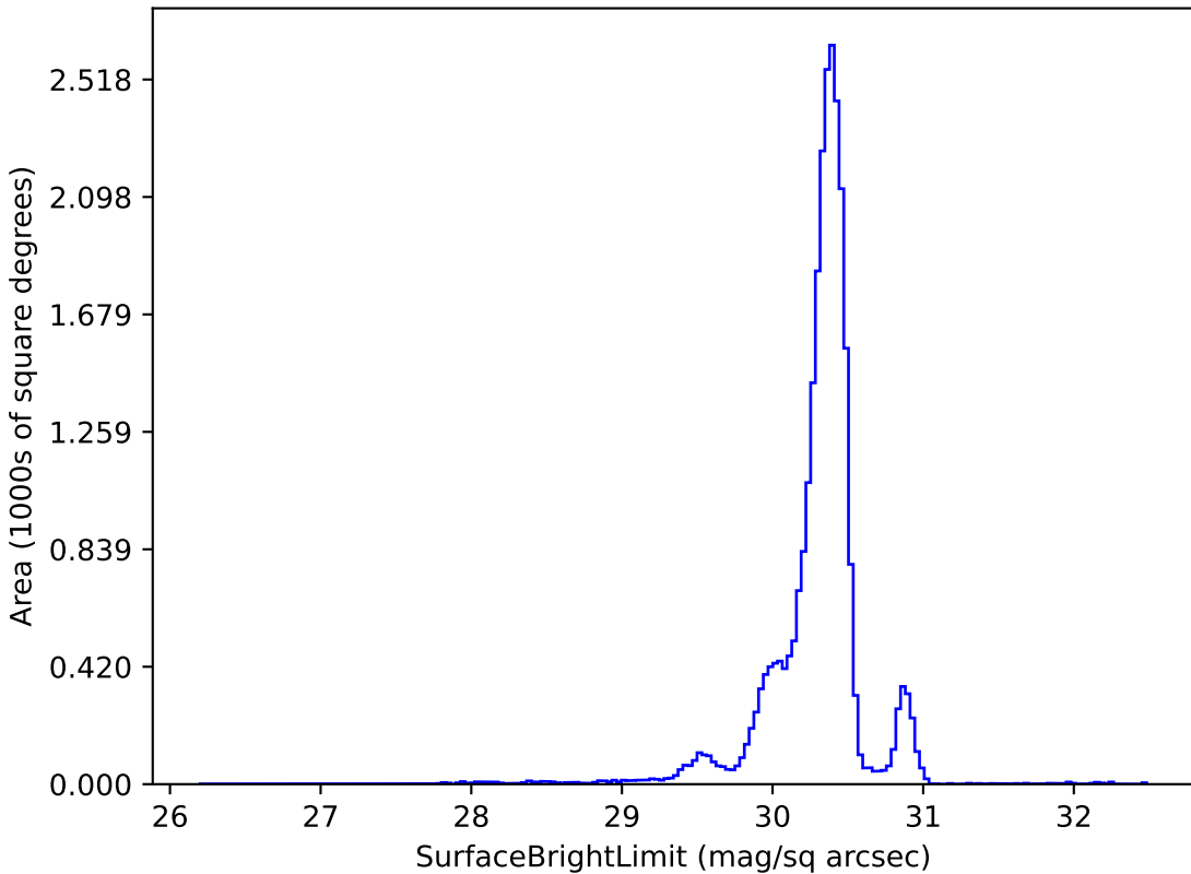
scp_reweight_v3.3_10yrs g: SurfaceBrightLimit
