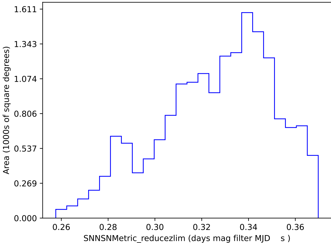
scp_reweight_v3.3_10yrs DDF excluded: SNNSNMetric_reducezlim
