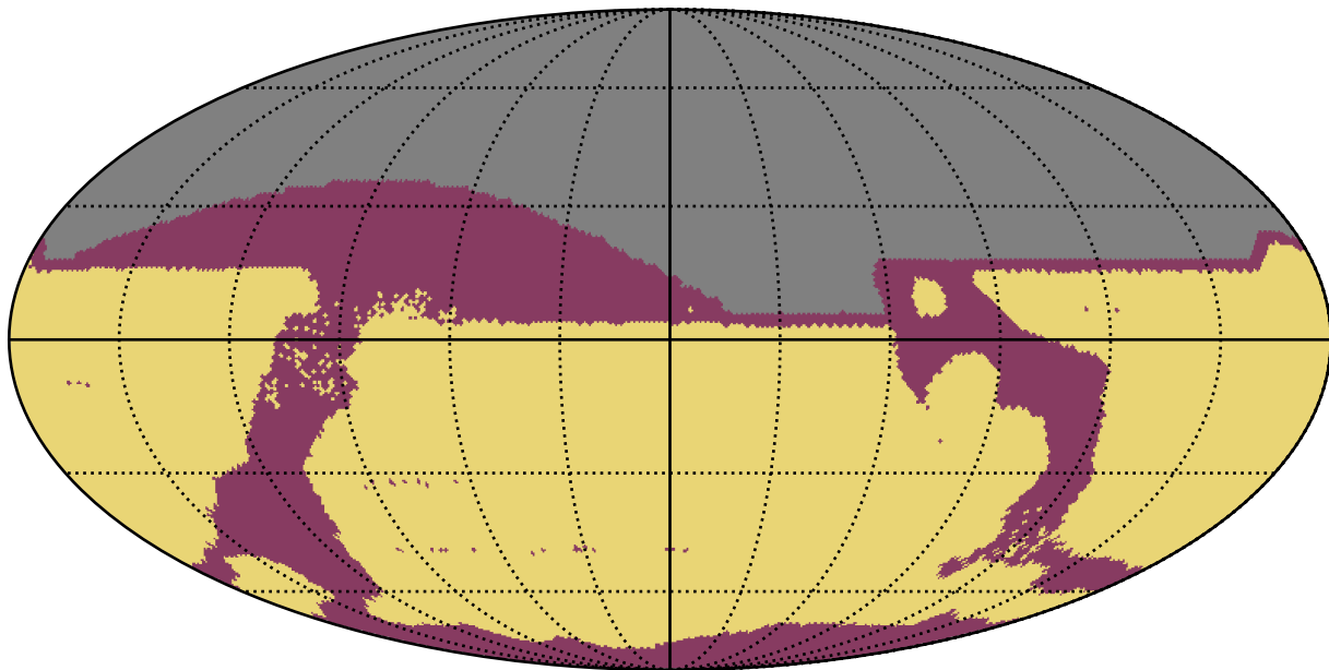
scp_reweight_v3.3_10yrs : RapidRevisits
