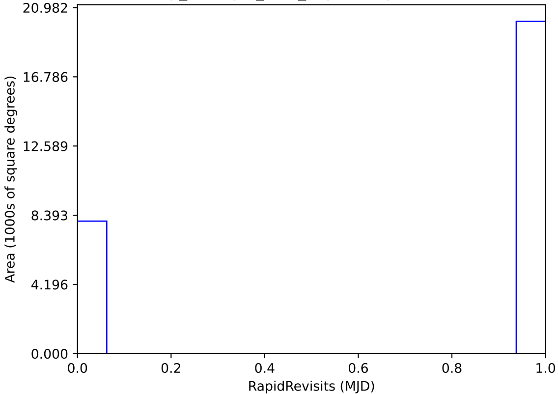
scp_reweight_v3.3_10yrs : RapidRevisits
