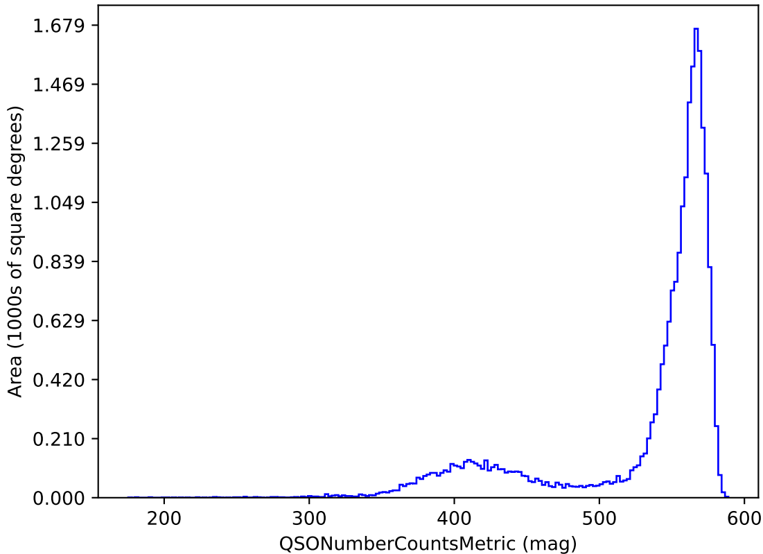
scp_reweight_v3.3_10yrs y band and non-DD: QSONumberCountsMetric
