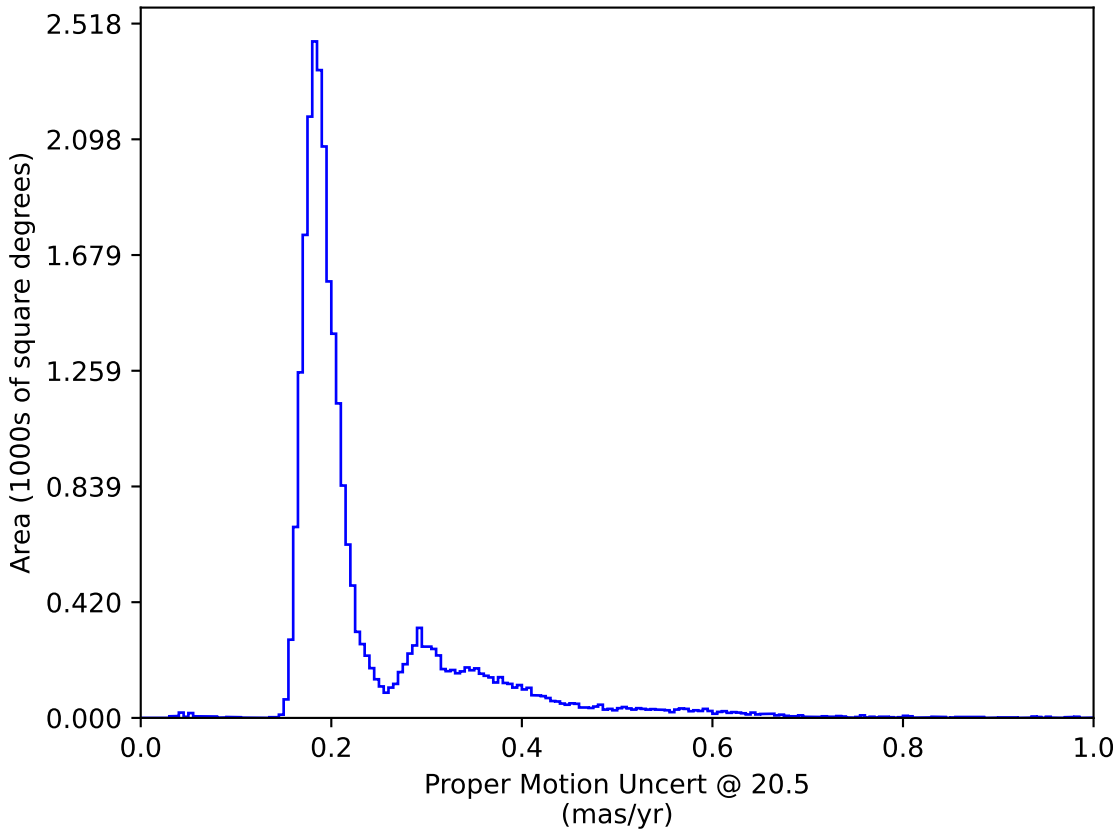
scp_reweight_v3.3_10yrs : Proper Motion Uncert @ 20.5
