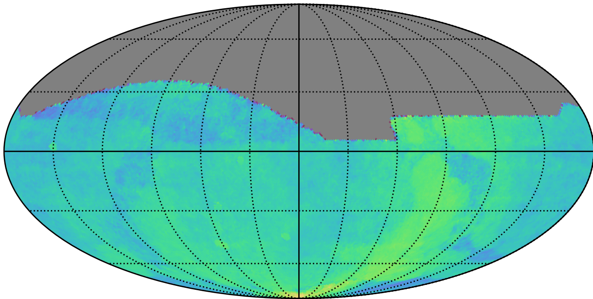
scp_reweight_v3.3_10yrs : Parallax Coverage @ 22.4
