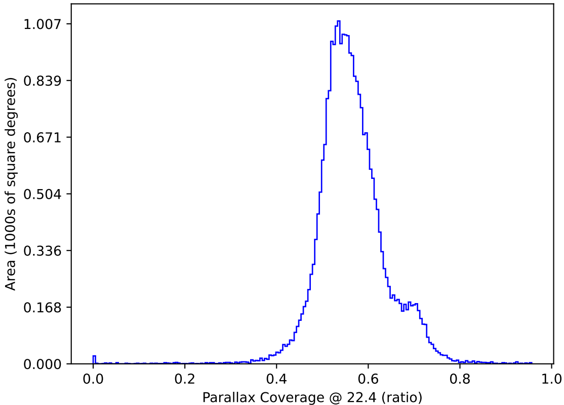
scp_reweight_v3.3_10yrs : Parallax Coverage @ 22.4
