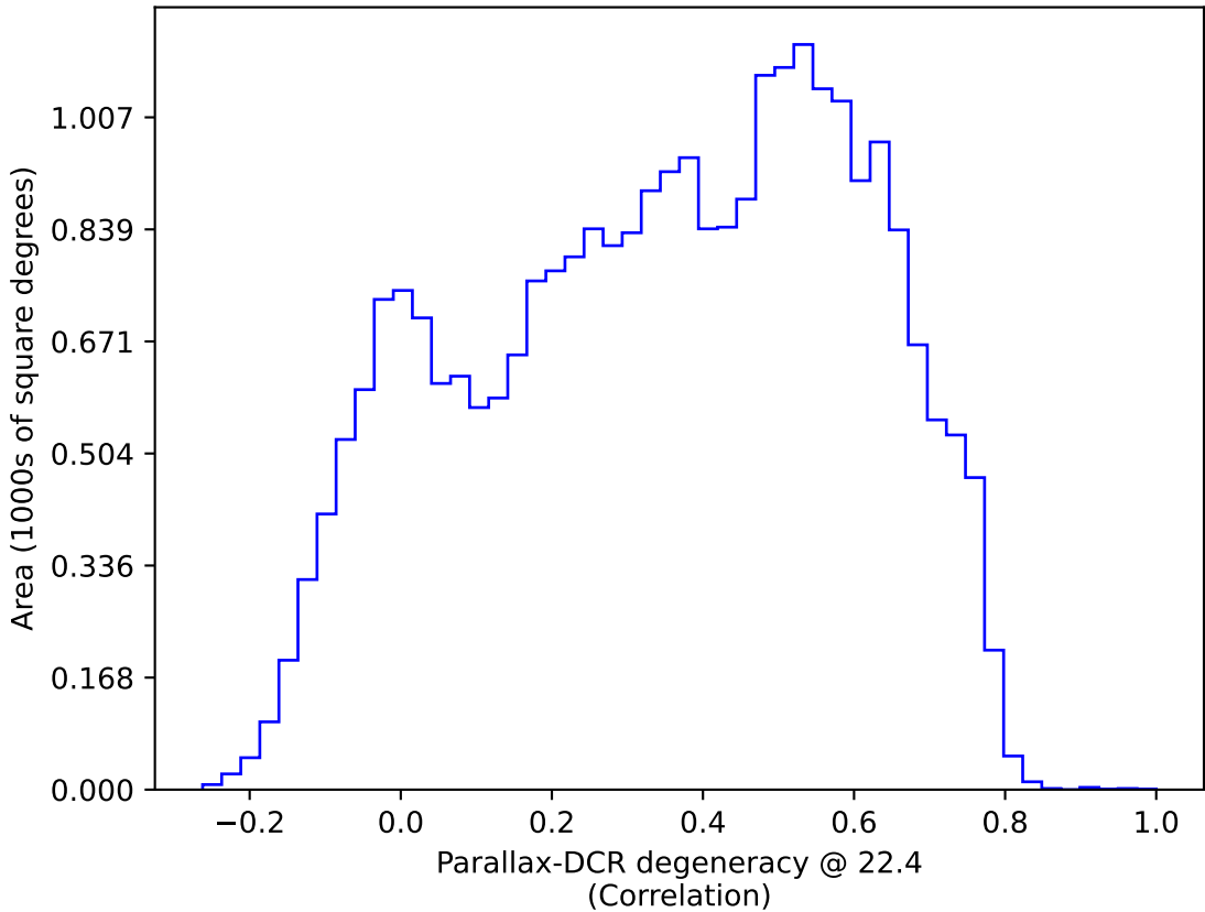
scp_reweight_v3.3_10yrs : Parallax-DCR degeneracy @ 22.4
