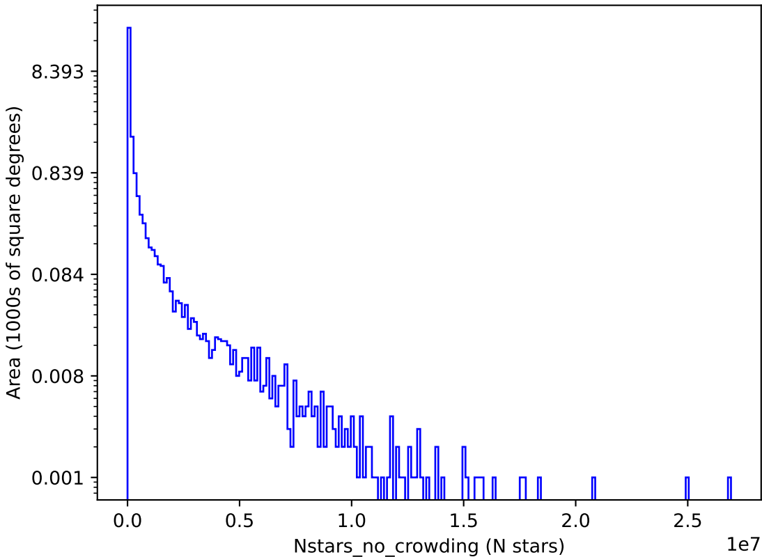
scp_reweight_v3.3_10yrs z: Nstars_no_crowding
