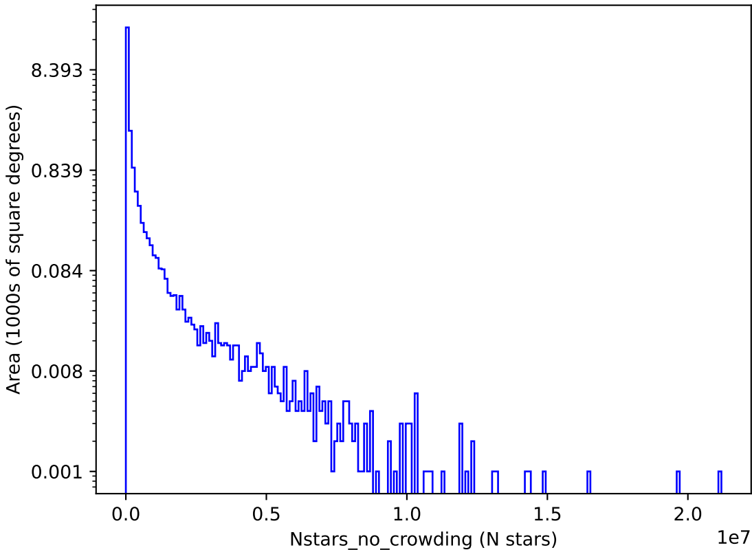
scp_reweight_v3.3_10yrs r: Nstars_no_crowding
