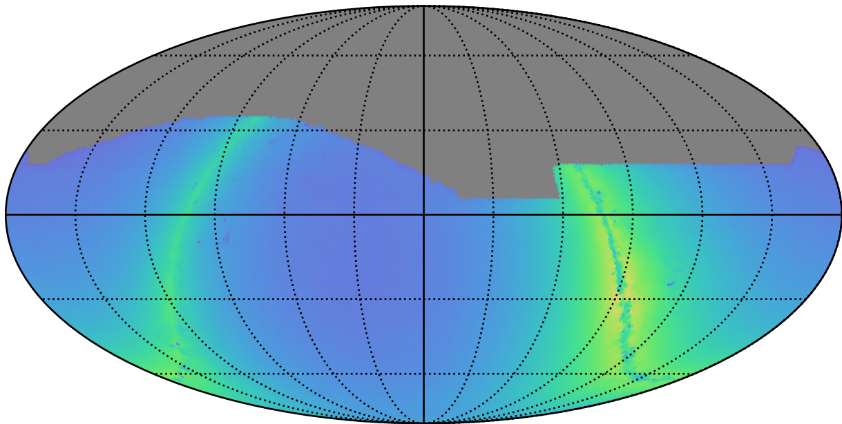
scp_reweight_v3.3_10yrs i: Nstars_no_crowding
