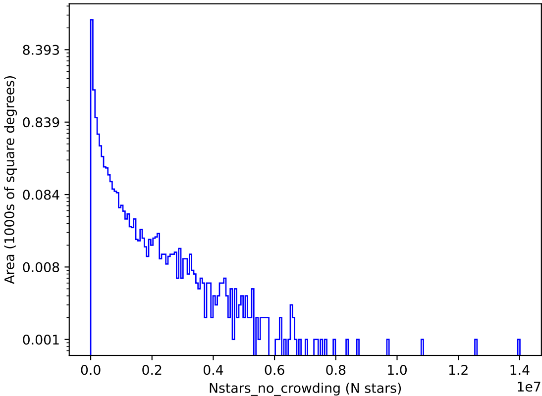
scp_reweight_v3.3_10yrs g: Nstars_no_crowding
