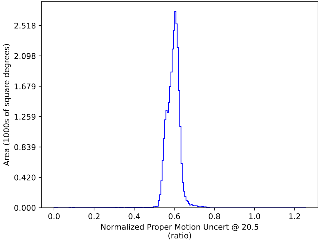
scp_reweight_v3.3_10yrs : Normalized Proper Motion Uncert @ 20.5
