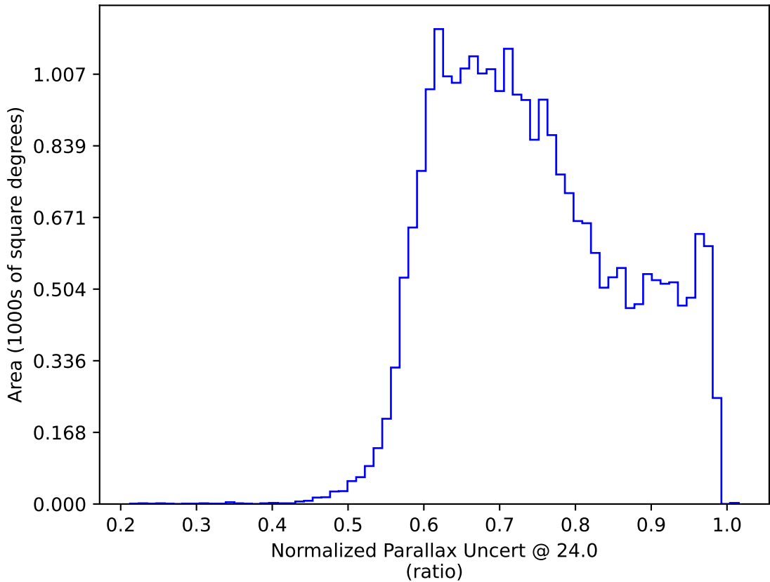
scp_reweight_v3.3_10yrs : Normalized Parallax Uncert @ 24.0
