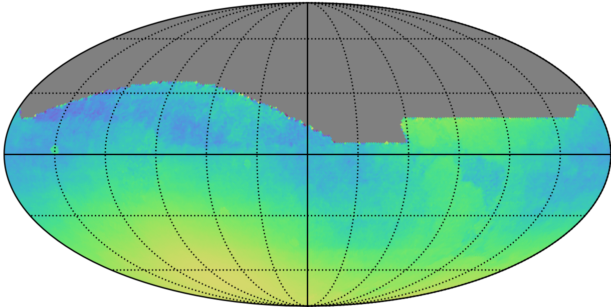
scp_reweight_v3.3_10yrs : Normalized Parallax Uncert @ 22.4
