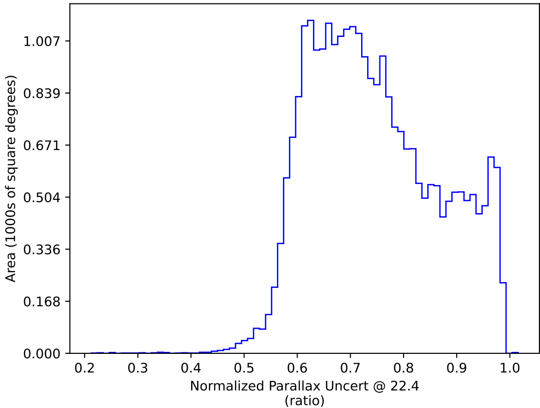
scp_reweight_v3.3_10yrs : Normalized Parallax Uncert @ 22.4
