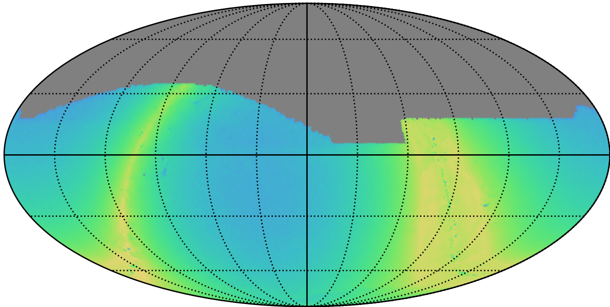
scp_reweight_v3.3_10yrs z: N stars to Precision 0.20
