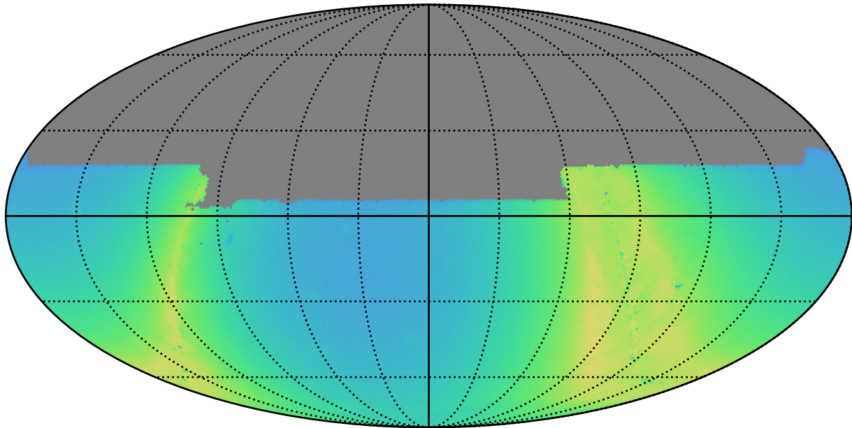
scp_reweight_v3.3_10yrs y: N stars to Precision 0.20
