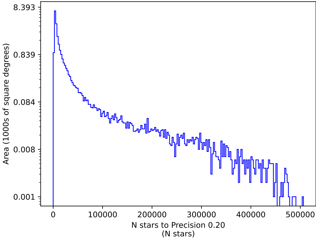
scp_reweight_v3.3_10yrs u: N stars to Precision 0.20
