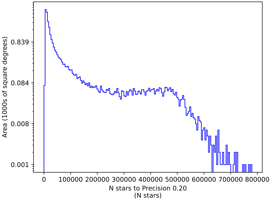
scp_reweight_v3.3_10yrs r: N stars to Precision 0.20
