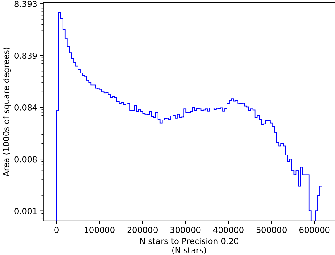
scp_reweight_v3.3_10yrs i: N stars to Precision 0.20
