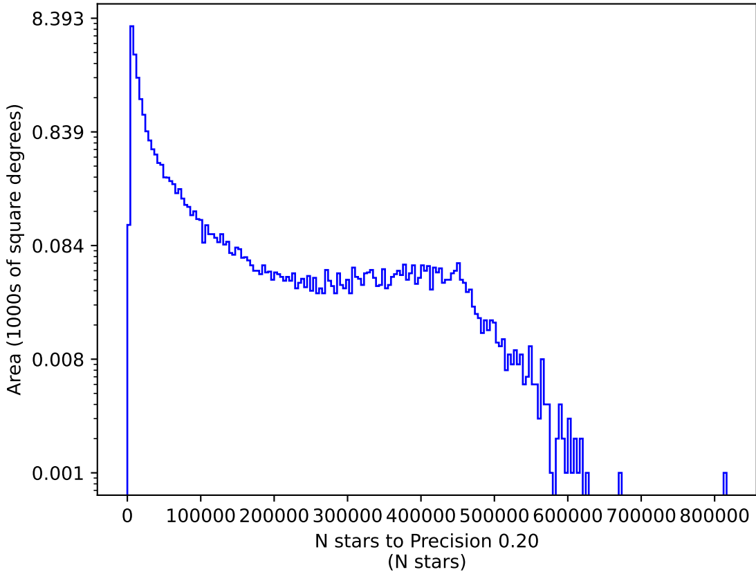
scp_reweight_v3.3_10yrs g: N stars to Precision 0.20
