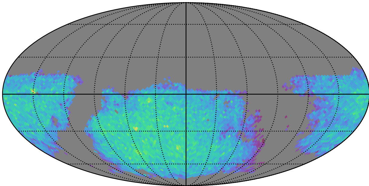
scp_reweight_v3.3_10yrs gi: LVDwarfs
