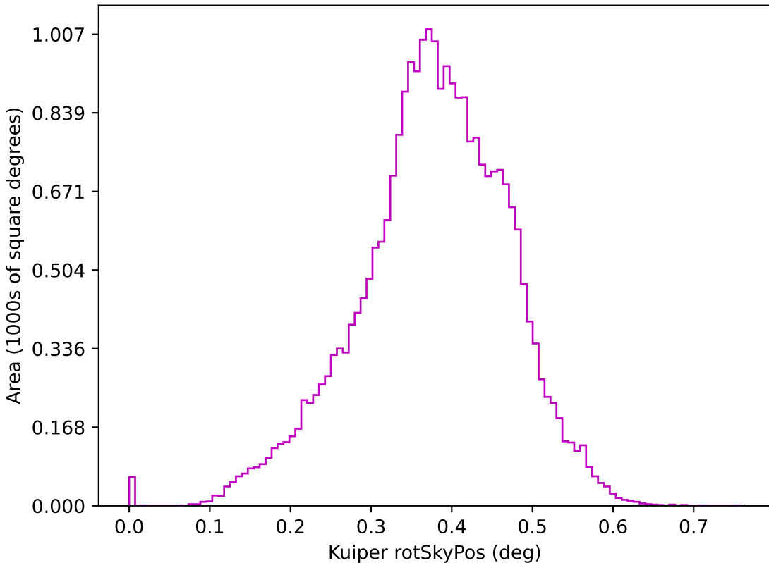
scp_reweight_v3.3_10yrs z: Kuiper rotSkyPos
