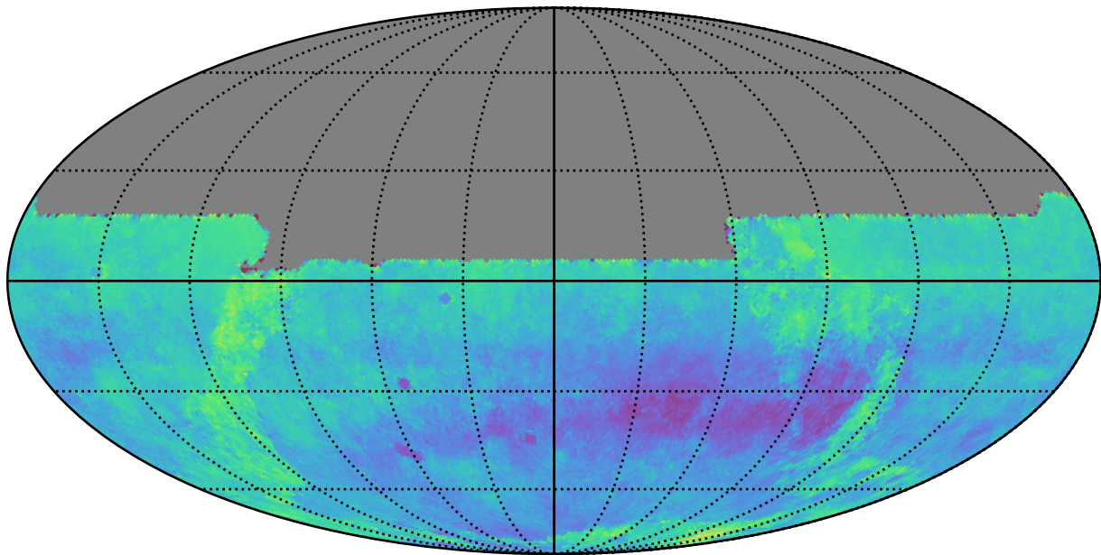
scp_reweight_v3.3_10yrs y: Kuiper rotSkyPos
