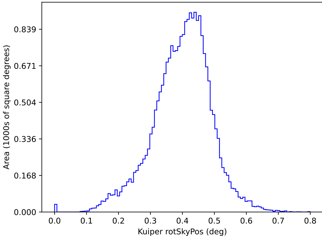
scp_reweight_v3.3_10yrs y: Kuiper rotSkyPos
