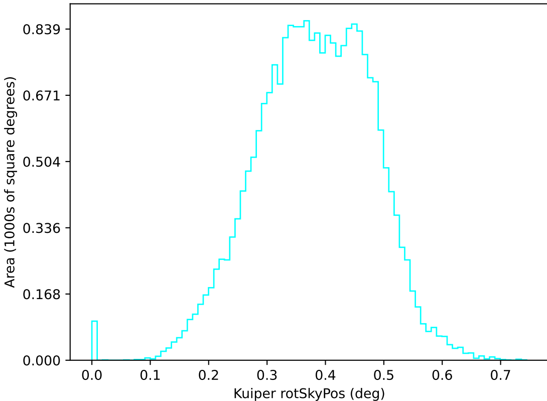
scp_reweight_v3.3_10yrs u: Kuiper rotSkyPos
