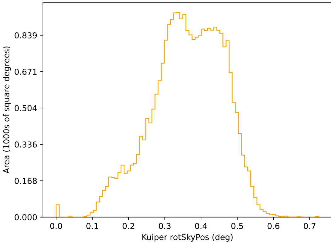
scp_reweight_v3.3_10yrs r: Kuiper rotSkyPos
