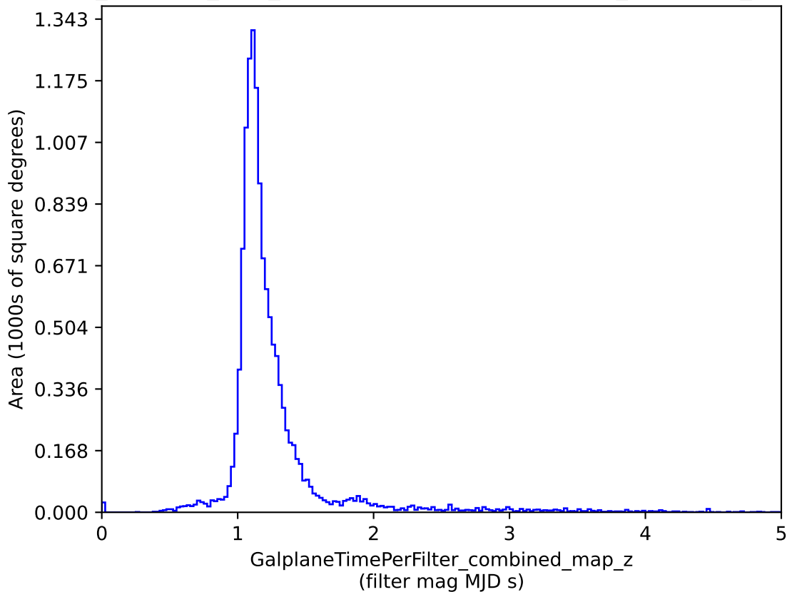
scp_reweight_v3.3_10yrs : GalplaneTimePerFilter_combined_map_z
