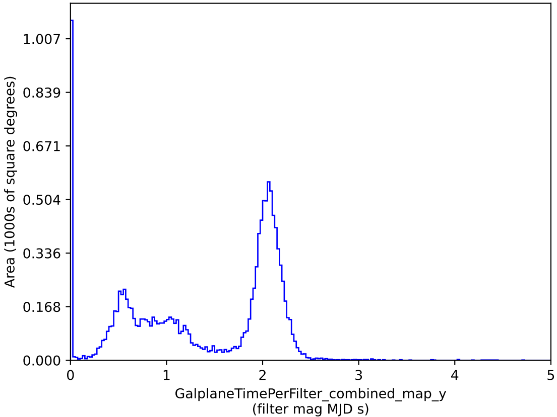
scp_reweight_v3.3_10yrs : GalplaneTimePerFilter_combined_map_y
