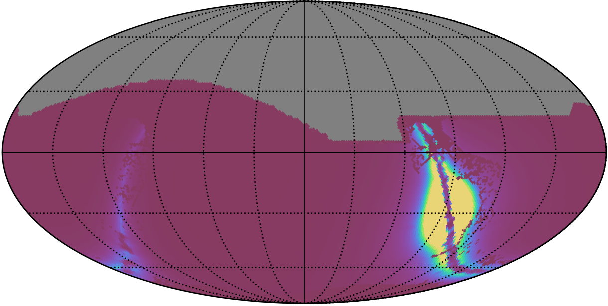
scp_reweight_v3.3_10yrs : GalplaneFootprintMetric_xray_binaries_map_Tau_20_0
