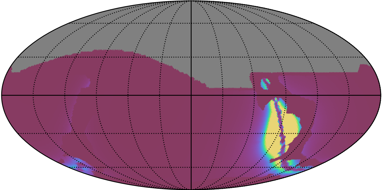
scp_reweight_v3.3_10yrs : GalplaneFootprintMetric_xray_binaries_map_Tau_11_0
