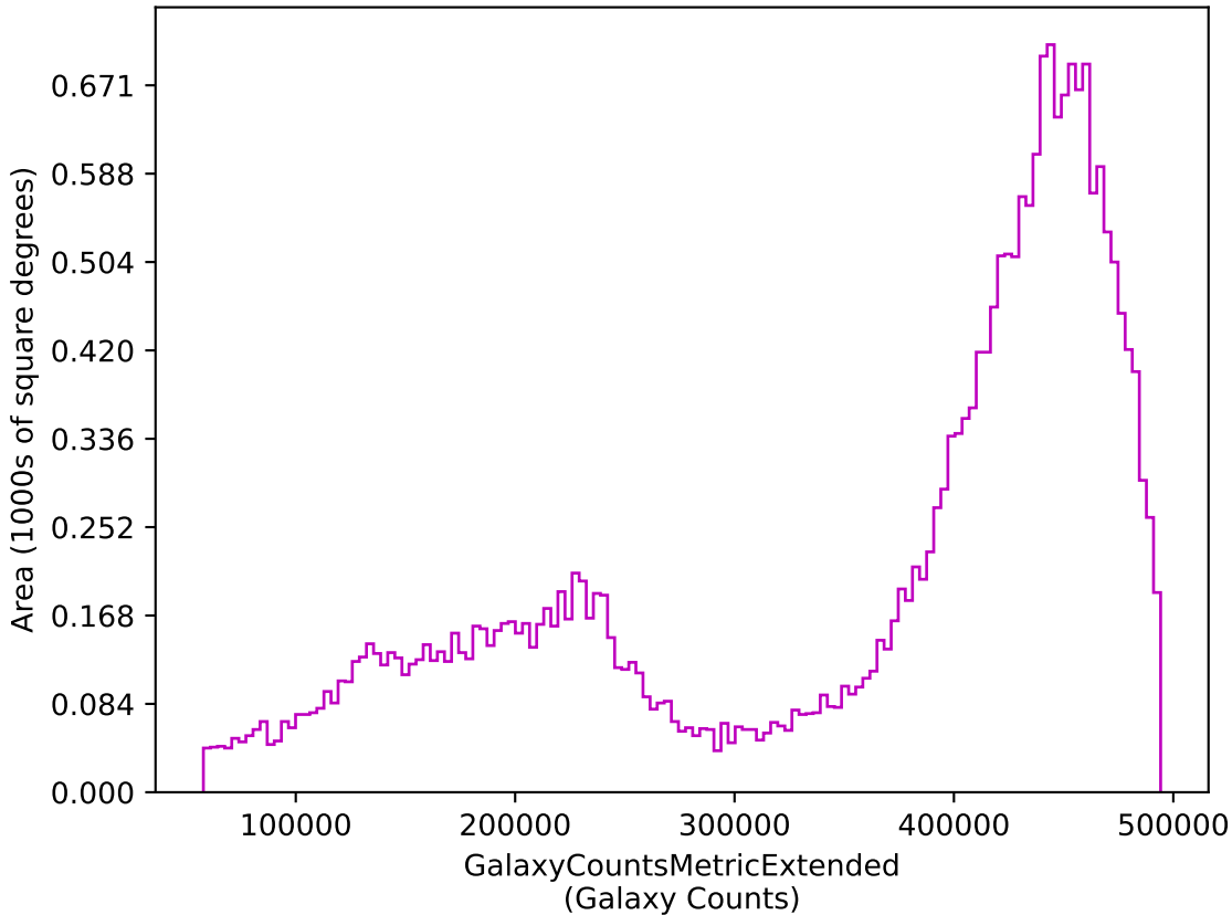
scp_reweight_v3.3_10yrs z: GalaxyCountsMetricExtended
