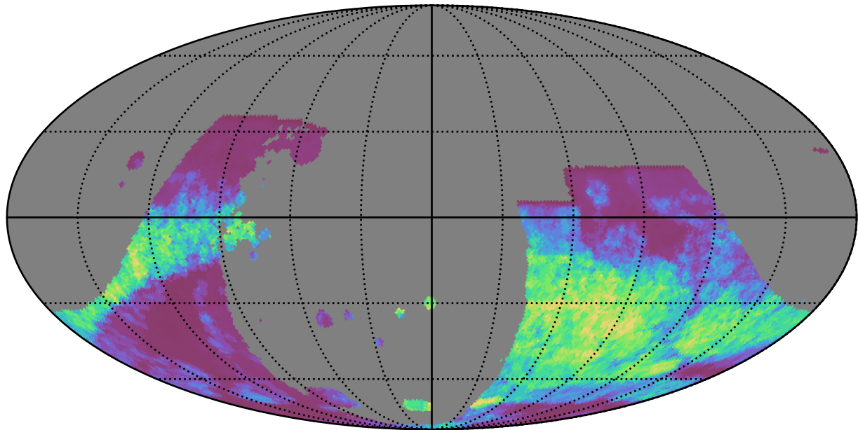
scp_reweight_v3.3_10yrs : GalPlaneSeasonGapsTimescales_combined_map_Tau_55_0
