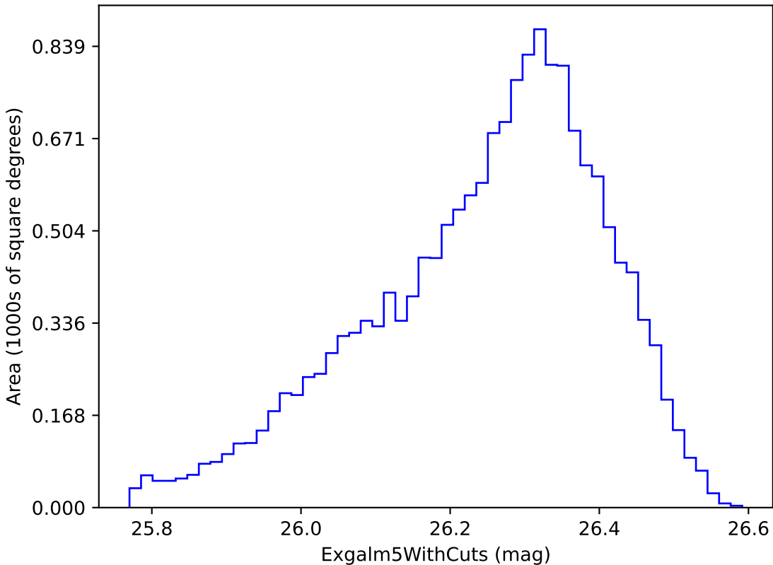
scp_reweight_v3.3_10yrs i band non-DD year 8: Exgalml5WithCuts
