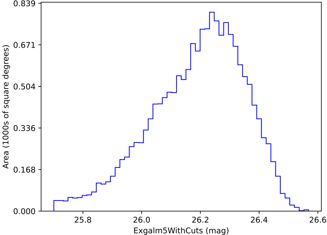
scp_reweight_v3.3_10yrs i band non-DD year 7: Exgal5WithCuts
