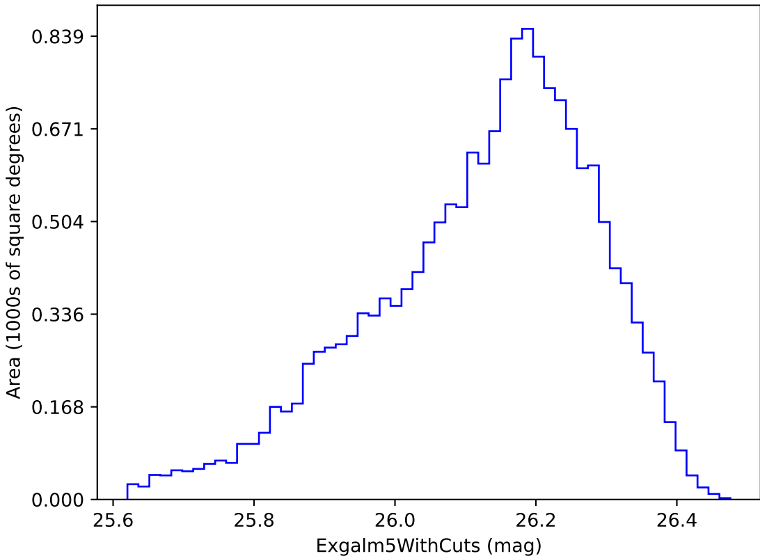
scp_reweight_v3.3_10yrs i band non-DD year 6: Exgalml5WithCuts
