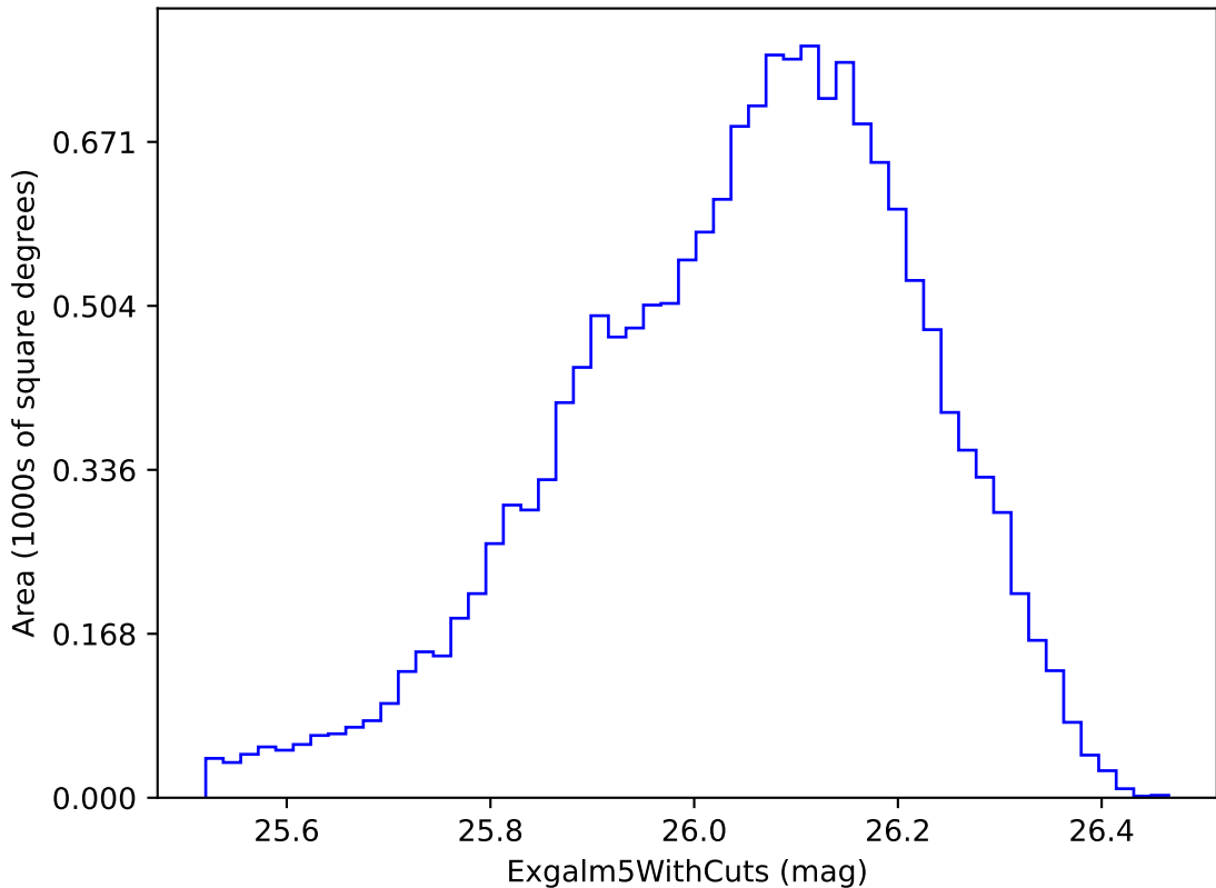
scp_reweight_v3.3_10yrs i band non-DD year 5: Exgal5WithCuts
