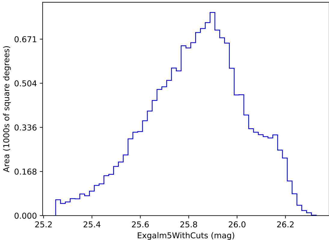
scp_reweight_v3.3_10yrs i band non-DD year 3: Exgalml5WithCuts
