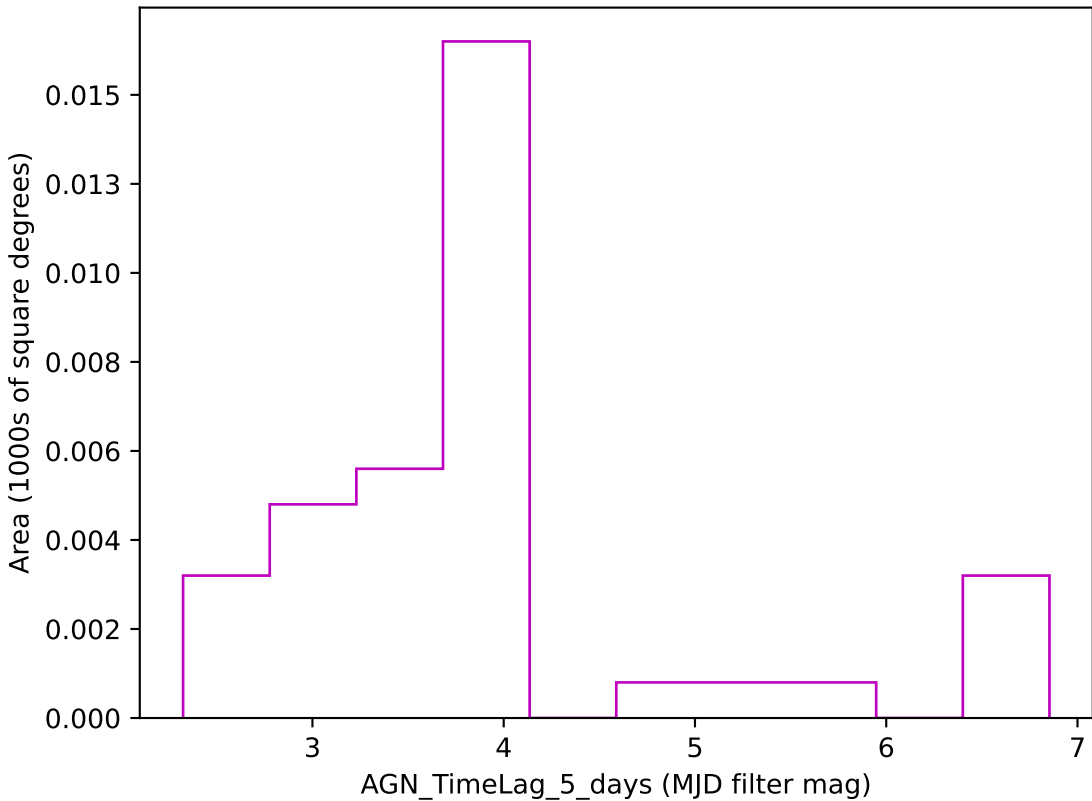
scp_reweight_v3.3_10yrs z band: AGN_TimeLag_5_days
