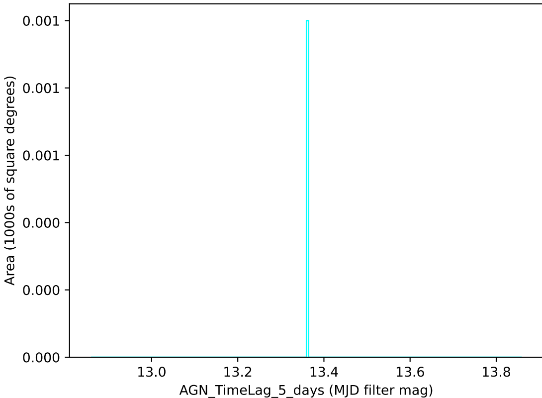
scp_reweight_v3.3_10yrs u band: AGN_TimeLag_5_days
