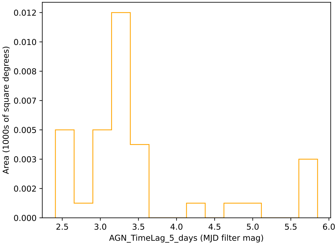
scp_reweight_v3.3_10yrs r band: AGN_TimeLag_5_days
